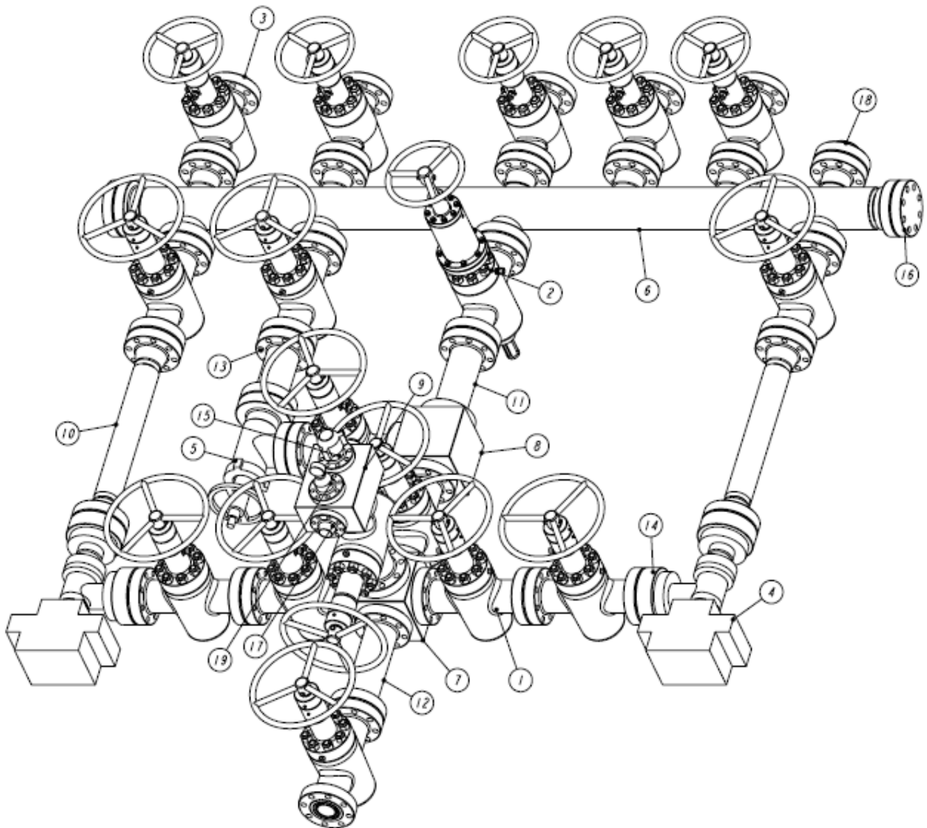
Example Choke Manifold
